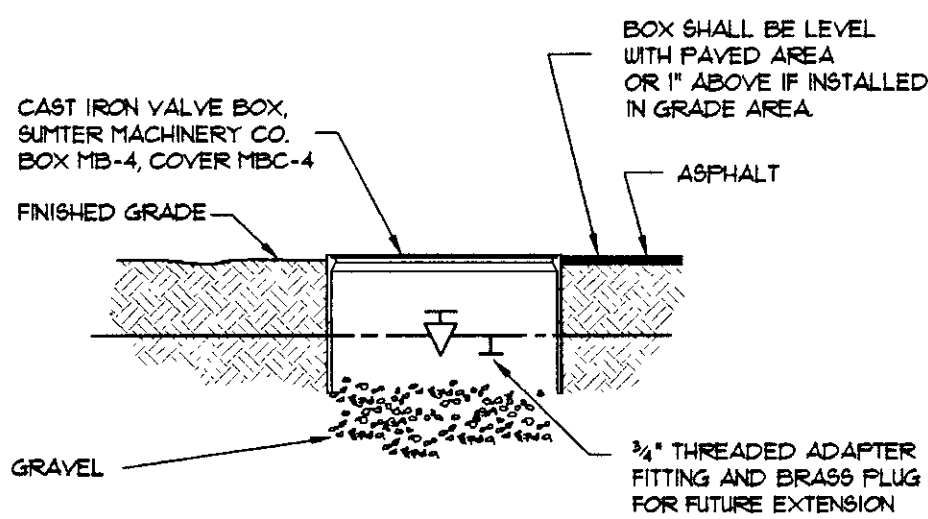
CUT-OFF VALVE BOX DETAIL
