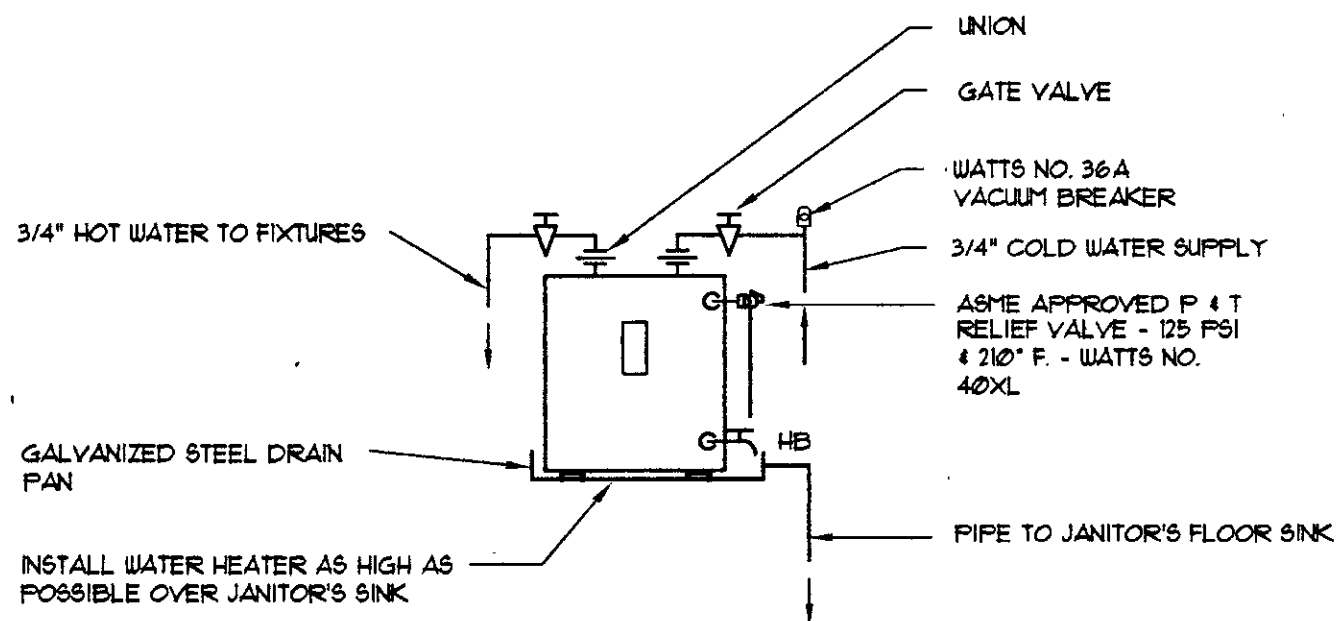
ELECTRIC WATER HEATER DETAIL
