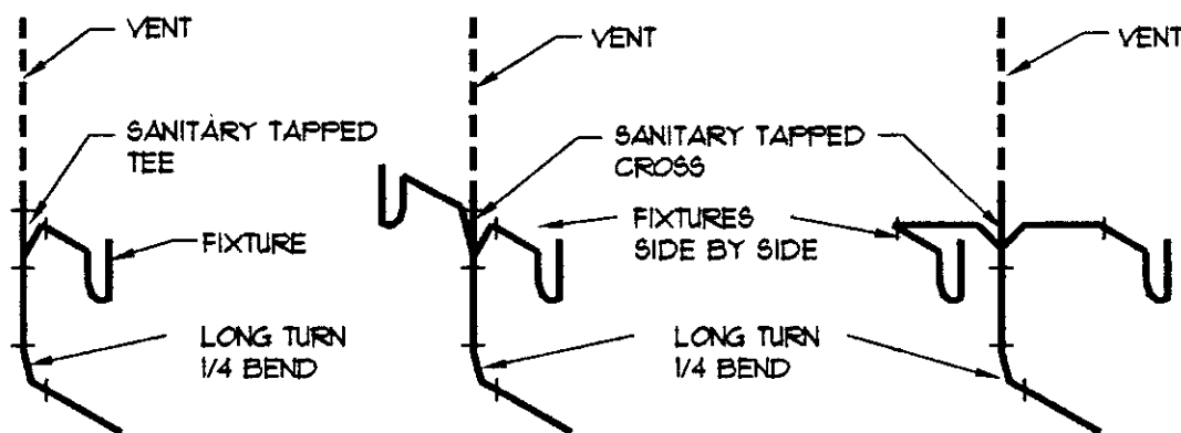
ROUGHING DIAGRAMS
