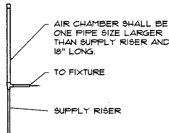
AIR CHAMBER DETAIL
