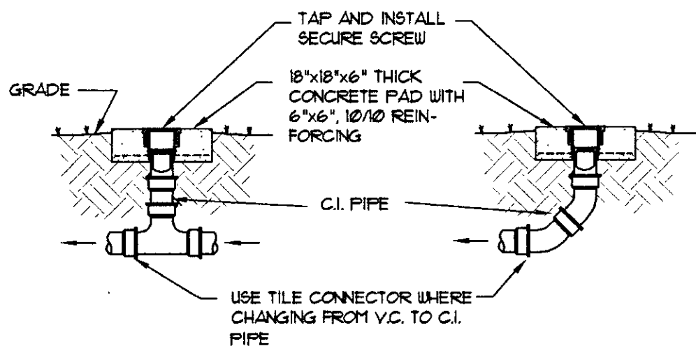
MIDDLE OF LINE END OF LINE CLEANOUT TO GRADE DETAIL
